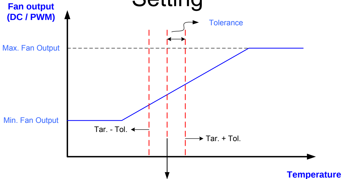
Figure 8-10 Setting of SMART FAN™ III
