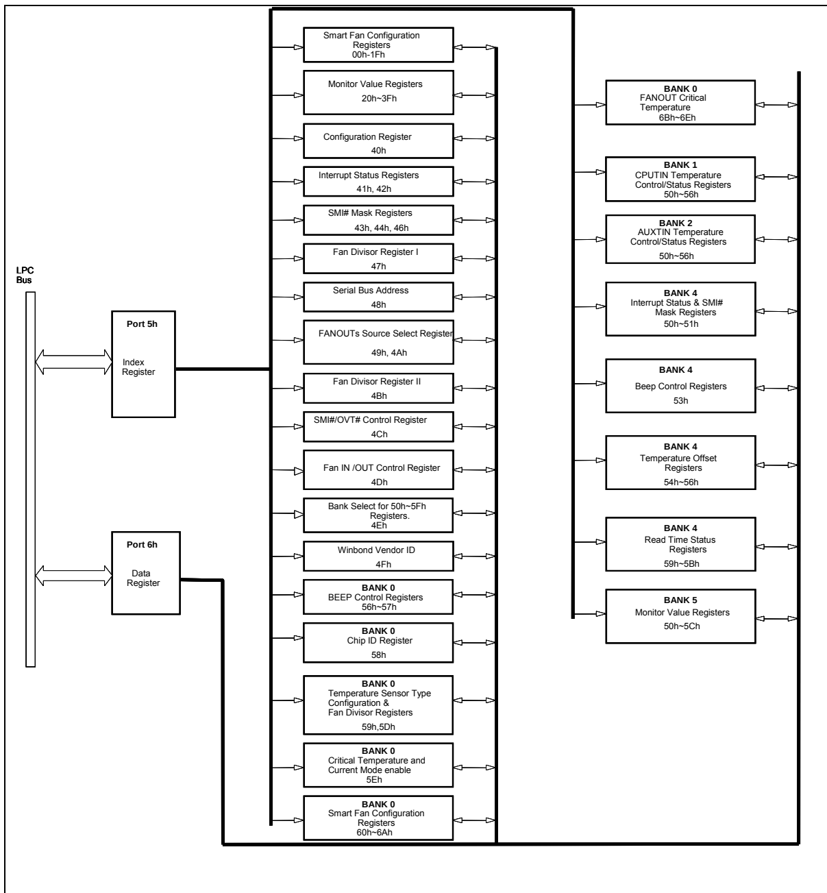
Figure 8-1 LPC Bus' Reads from / Write to Internal Registers
