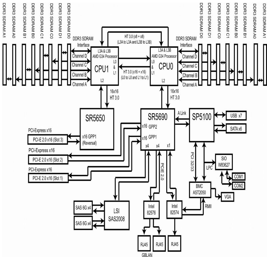
S8236-IL Block Diagram
