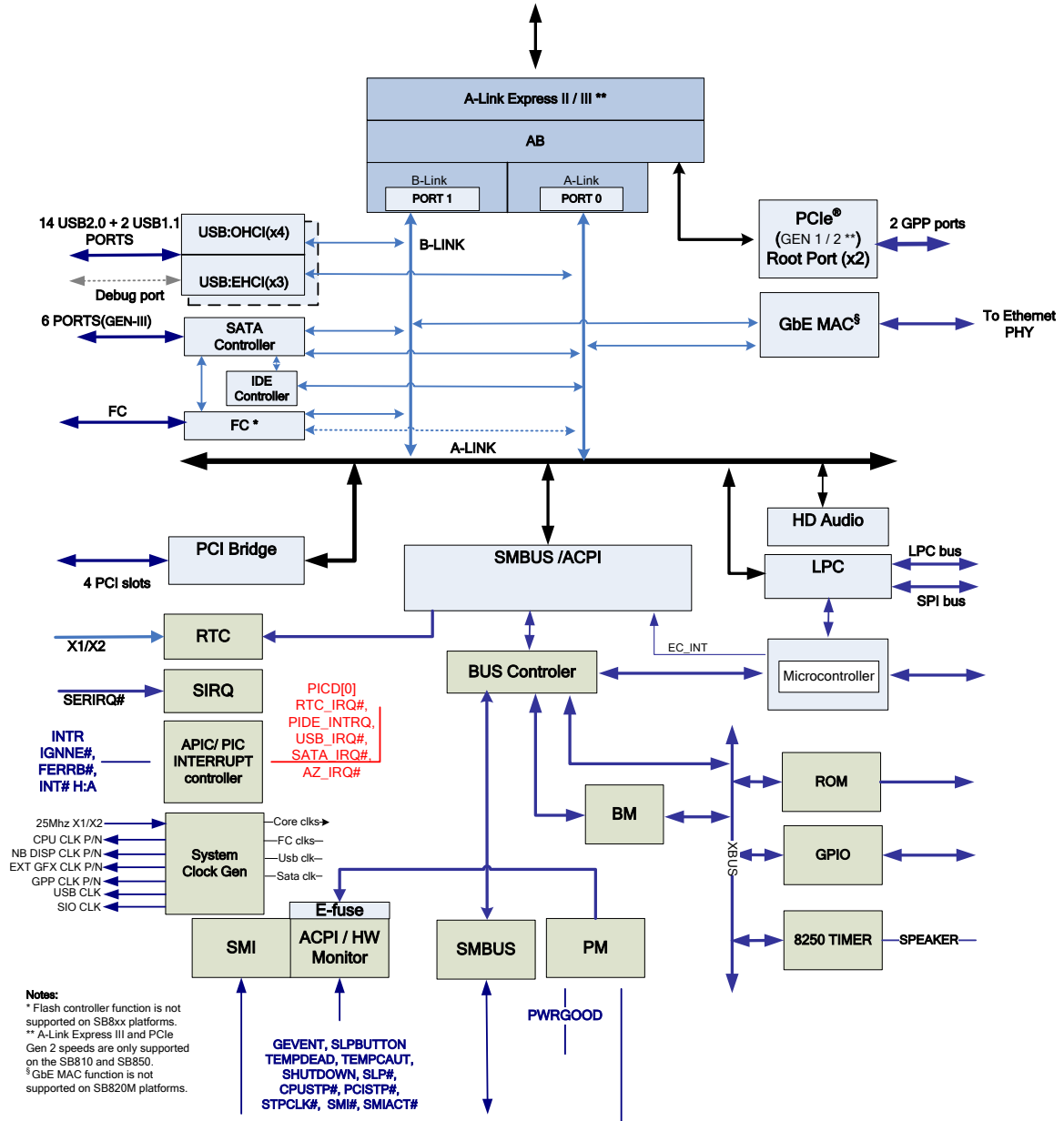
Figure 1 SB800 Internal PCI Devices and Major Functional Blocks
