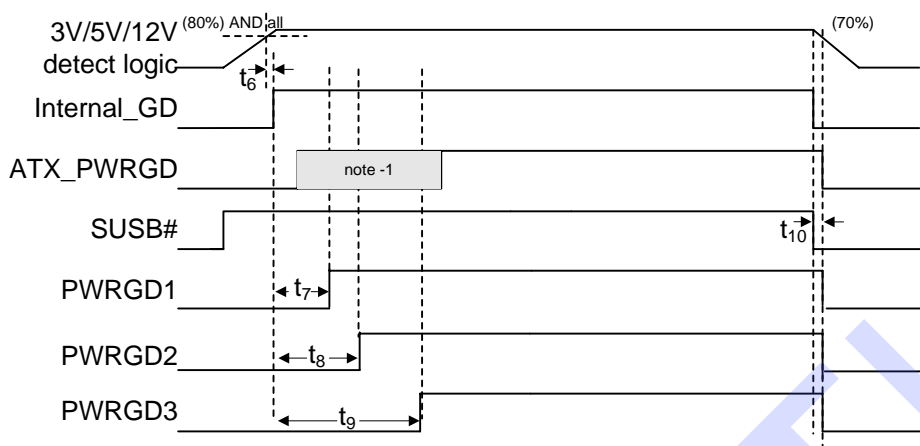
Figure 11-16. PWRGD1/2/3 Signal Timings
