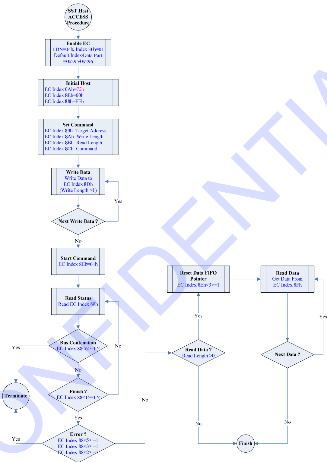
Figure 9-8. SST Host Programming Procedure
