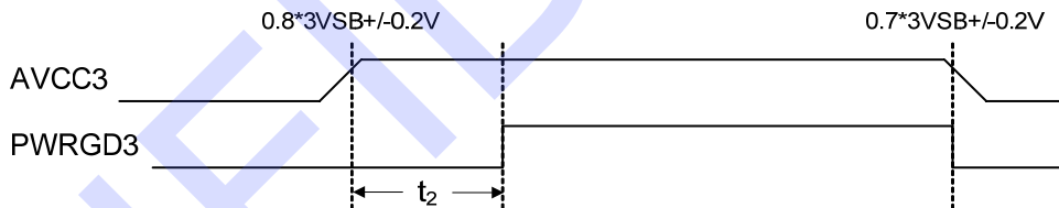
Figure 11-13. PWRGD3 Timings
