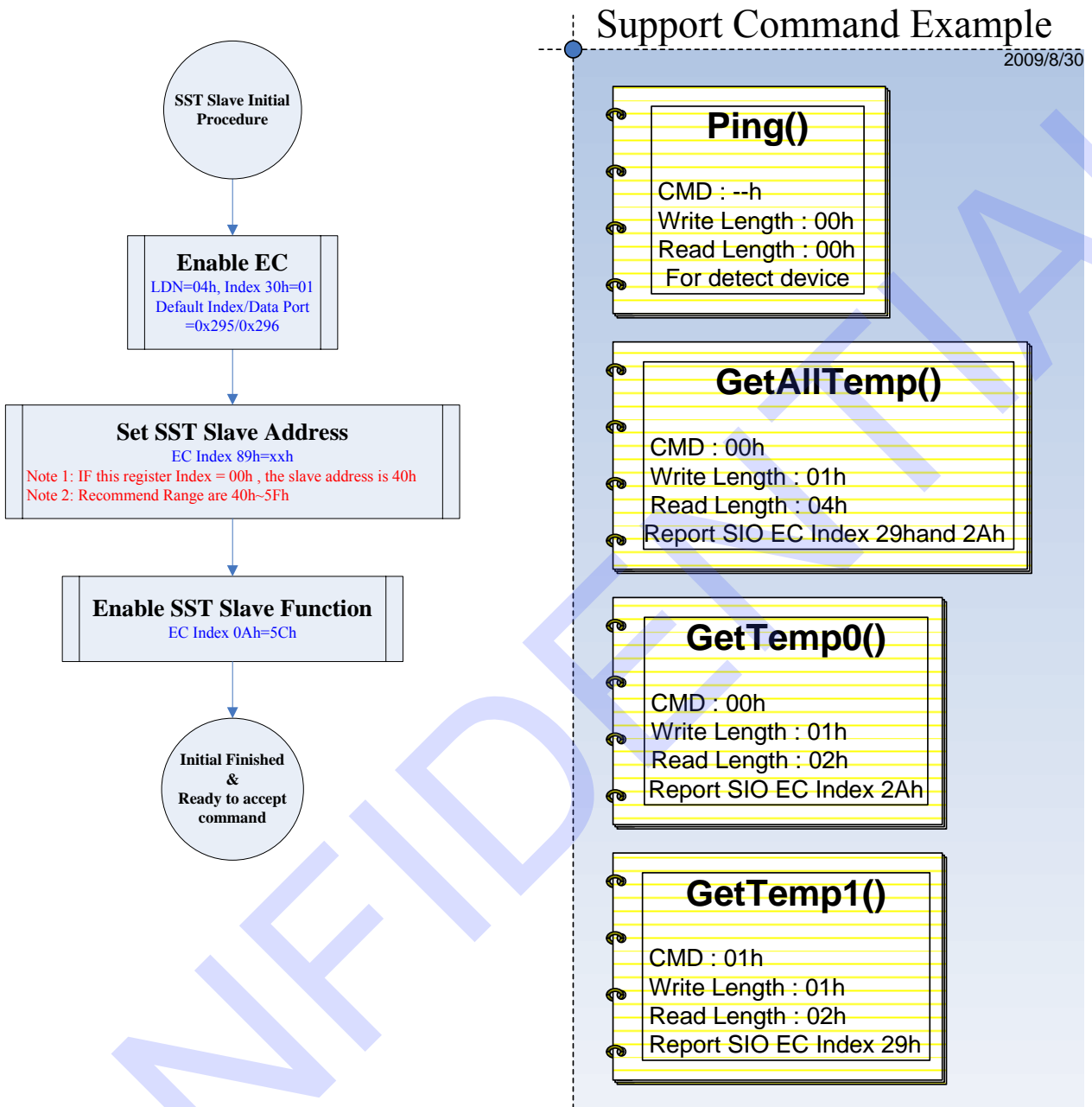
Figure 9-10. SST Slave Programming Procedure
