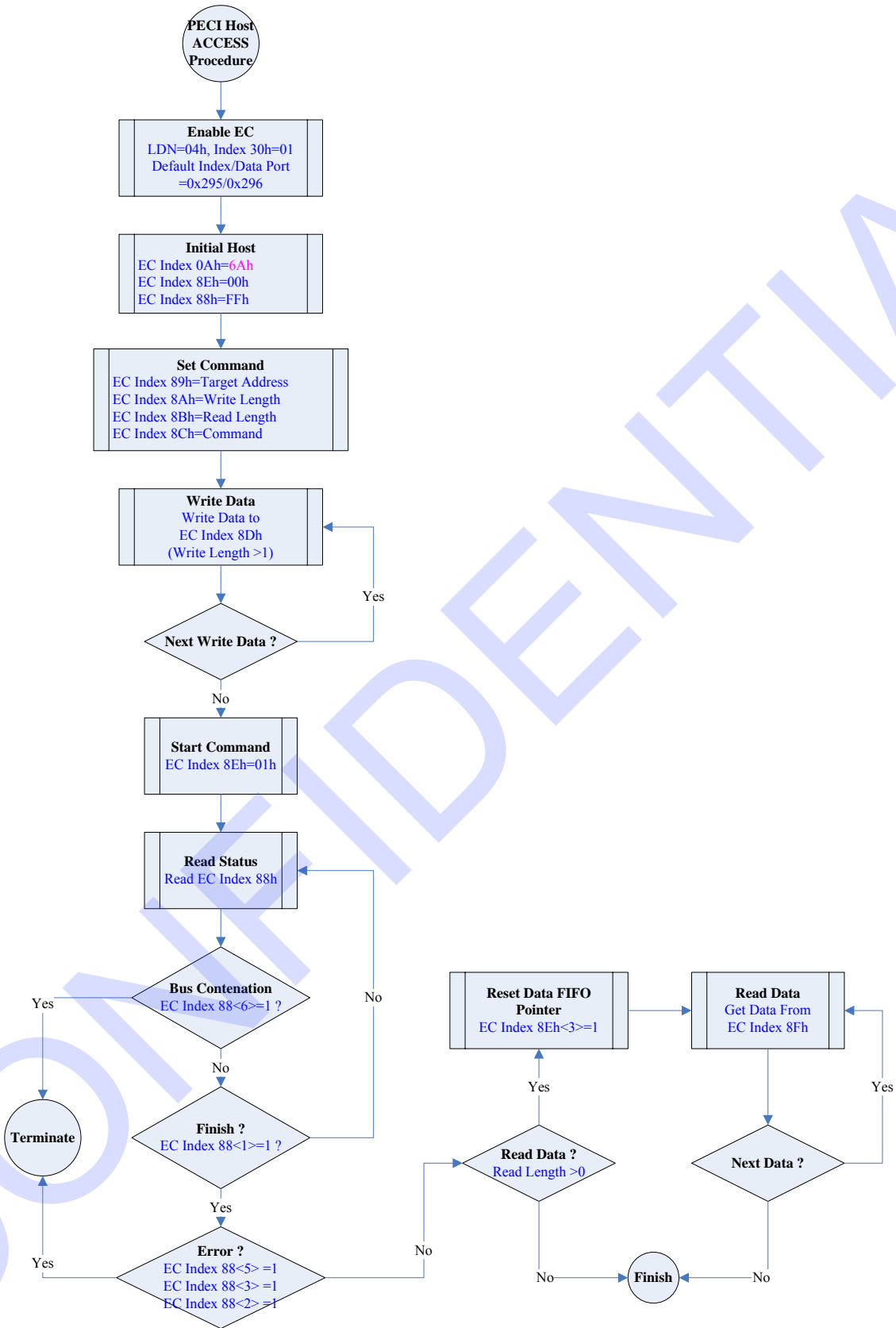
Figure 9-9. PECE Host Programming Procedure
