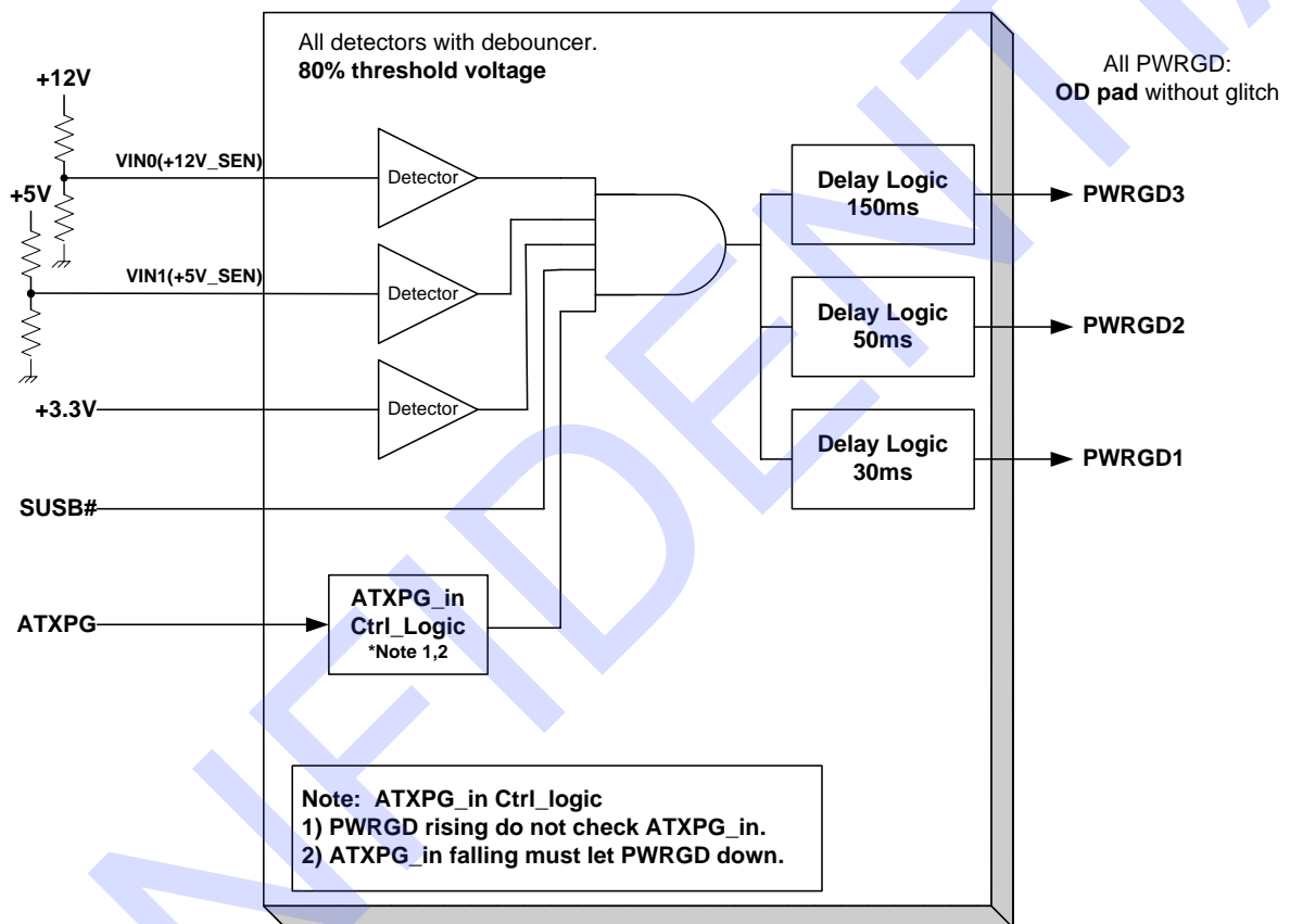
Figure 11-15. PWRGD1/2/3 Signal Condition
