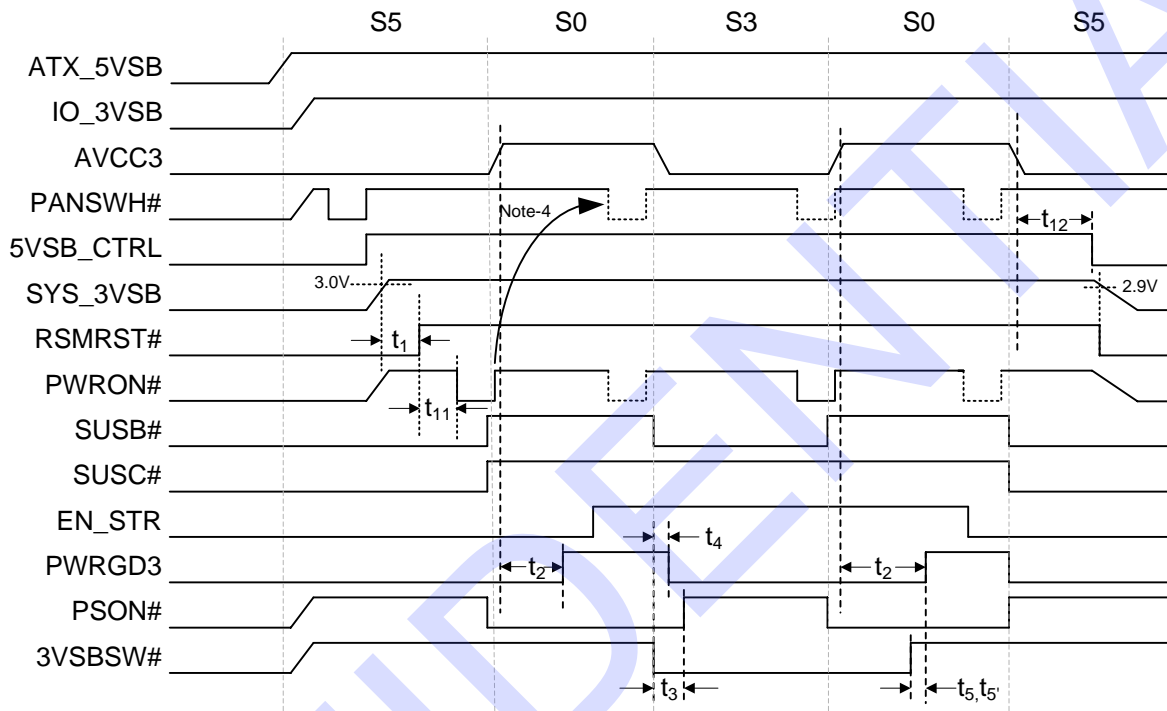
Figure 11-17. EuP Function Signal Timings
