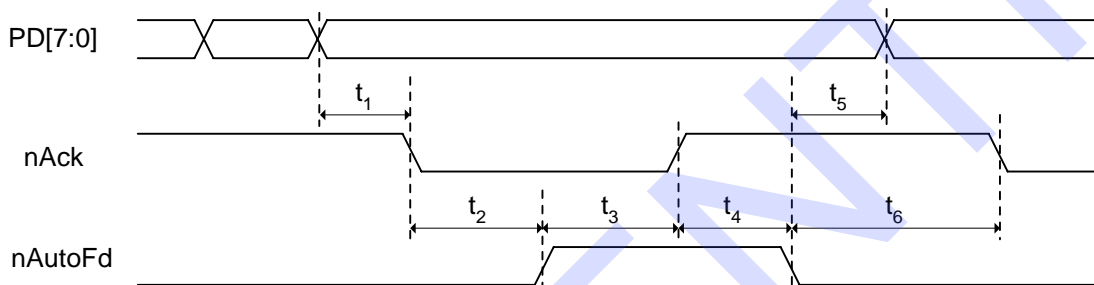
Figure 11-11. ECP Parallel Port Backward Timings
