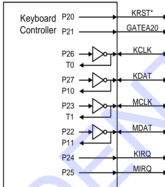
Figure 9-12. Keyboard and Mouse Interface
