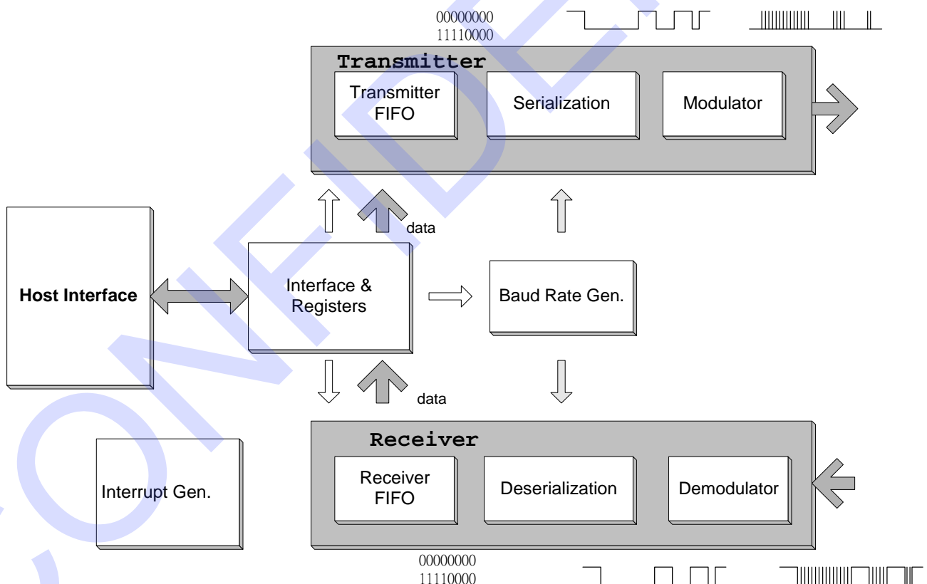
Figure 9-13. CIR Block Diagram
