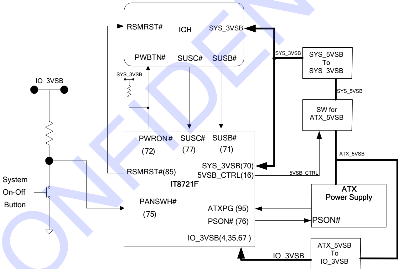
Figure 7-1. IT8721F Special Applications Circuitry for Intel ICH
