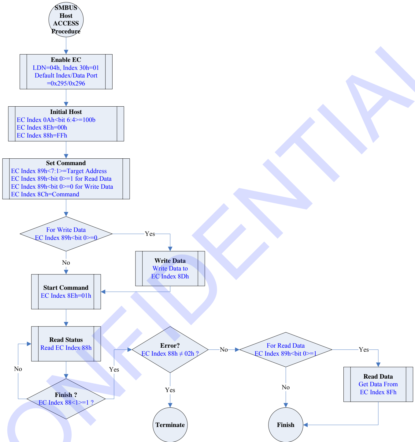
Figure 9-11. SMBus Host Slave Programming Procedure
