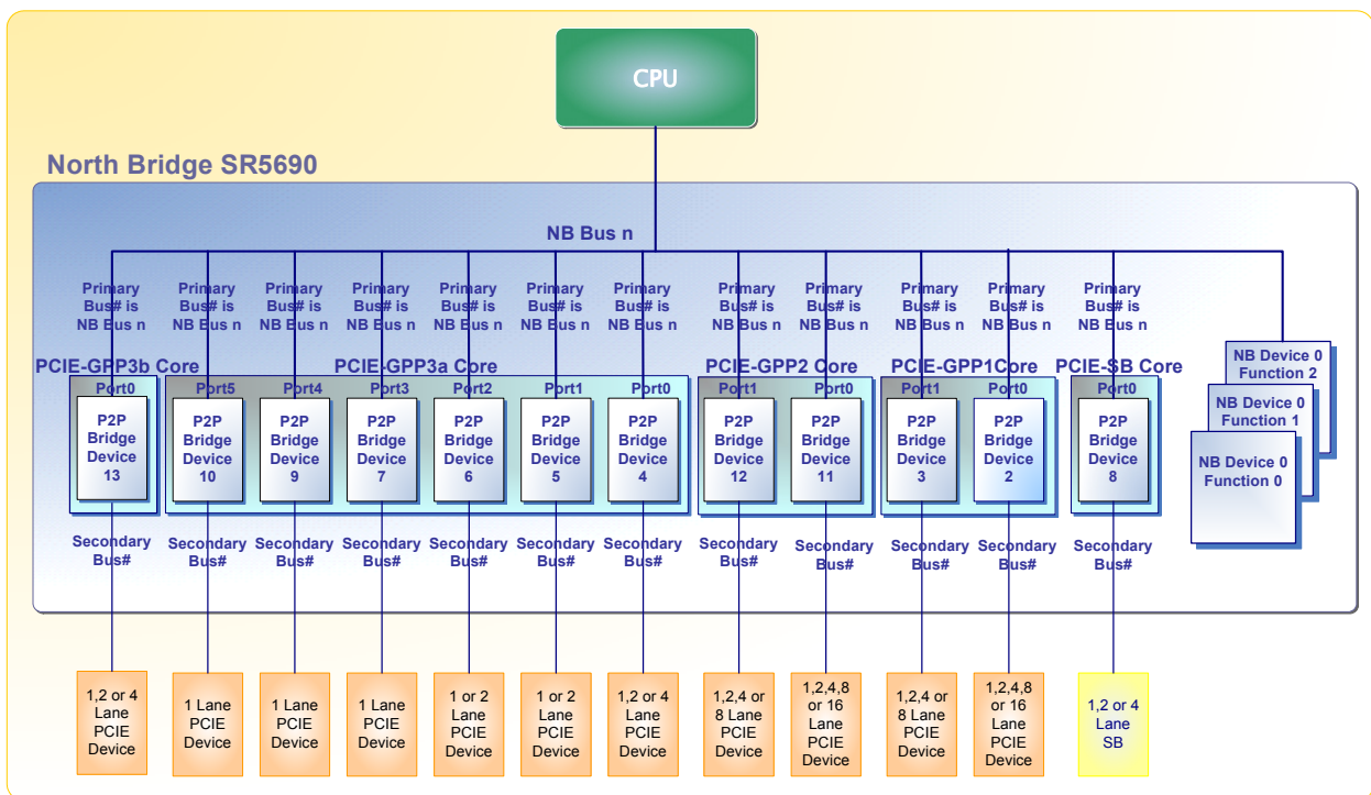
Figure 4-1 SR5690 PCIe® Configuration Space Topology
